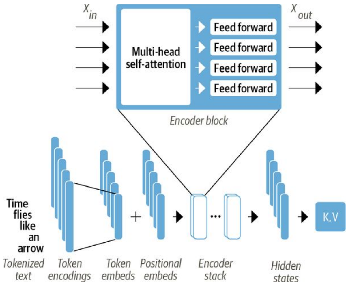
Figure 3-2. Zooming into the encoder layer
