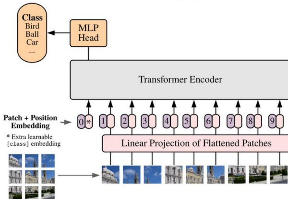
Figure 11-9. The ViT architecture (courtesy of Alexey Dosovitskiy et al.)
