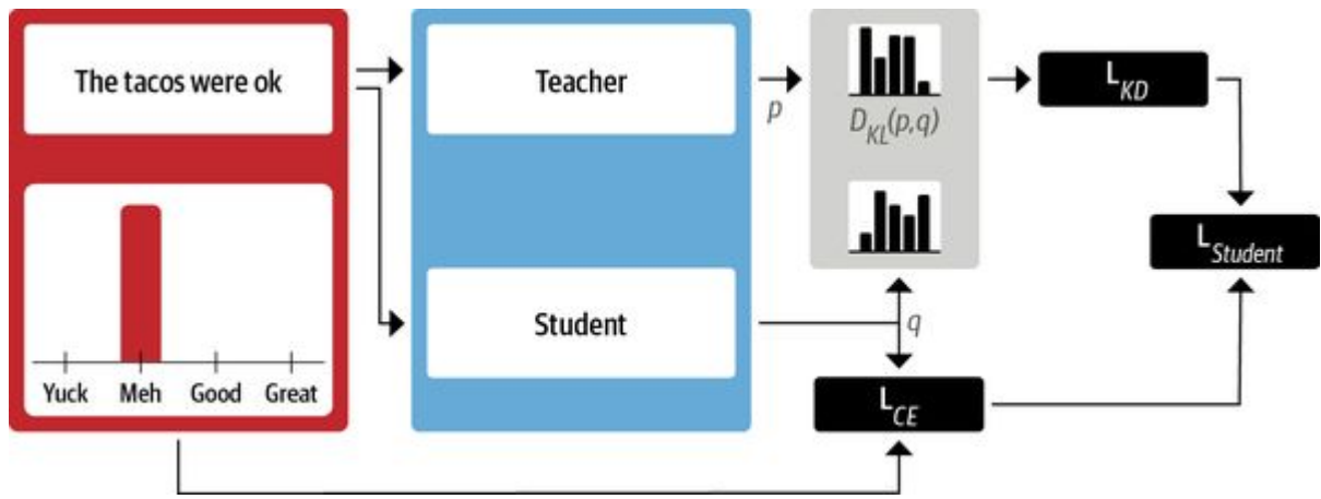
Figure 8-4. The knowledge distillation process
