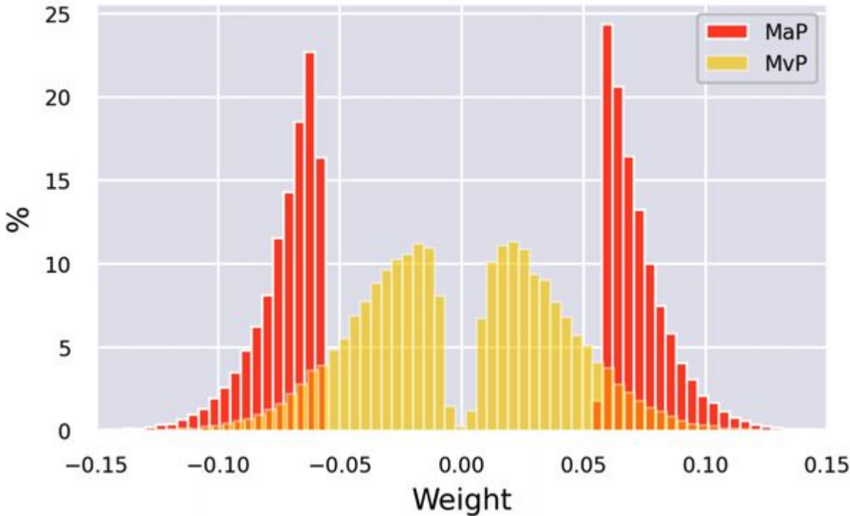
Figure 8-13. Distribution of remaining weights for magnitude pruning (MaP) and movement pruning (MvP)
