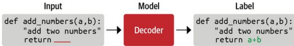
Figure 10-2. In causal language modeling, the future tokens are masked and the model has to predict them; typically a decoder model such as GPT is used for such a task
