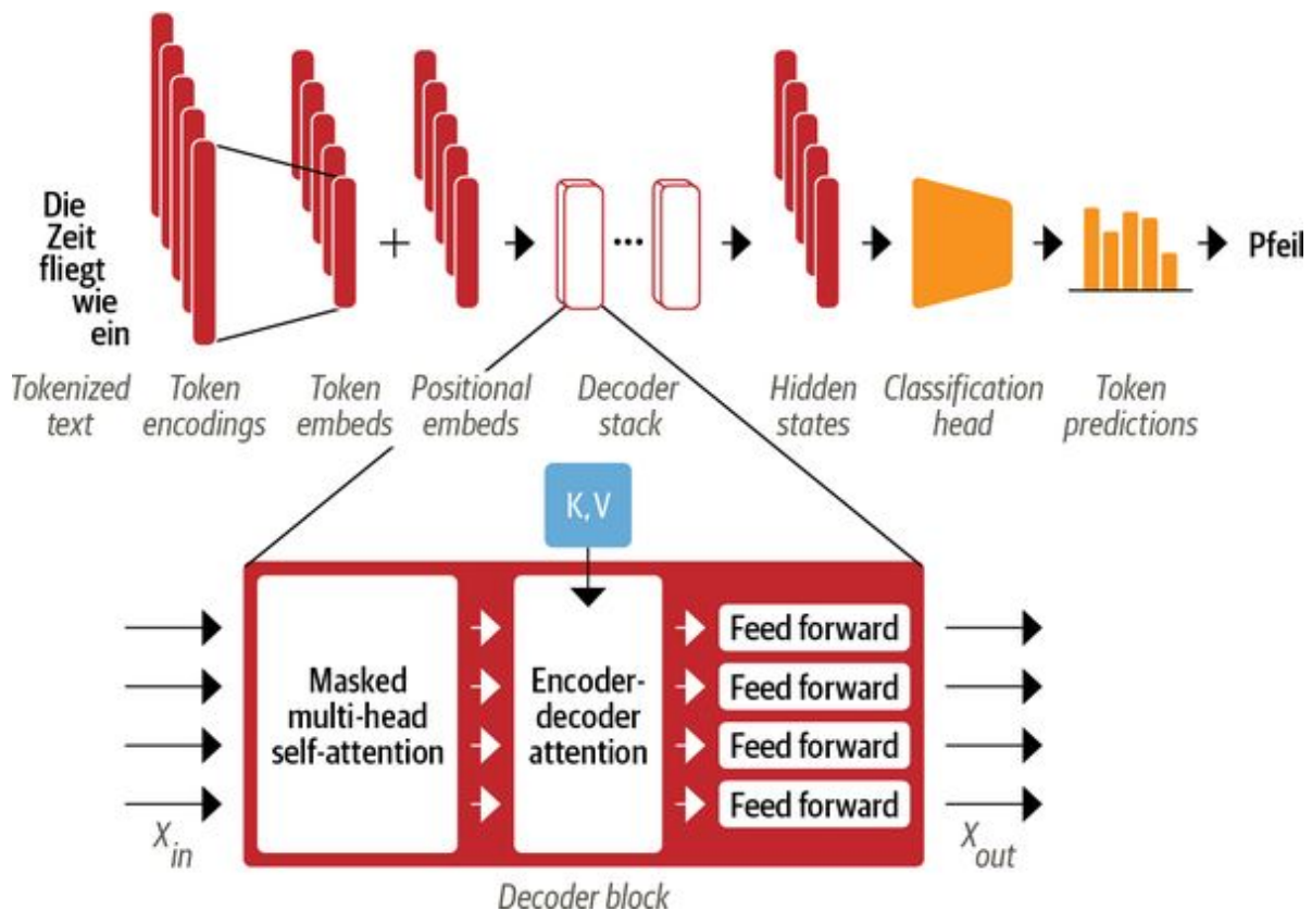
Figure 3-7. Zooming into the transformer decoder layer
