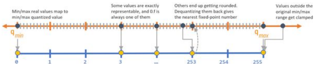
Figure 8-6. Quantizing floating-point numbers as unsigned 8-bit integers (courtesy of Manas Sahni)
