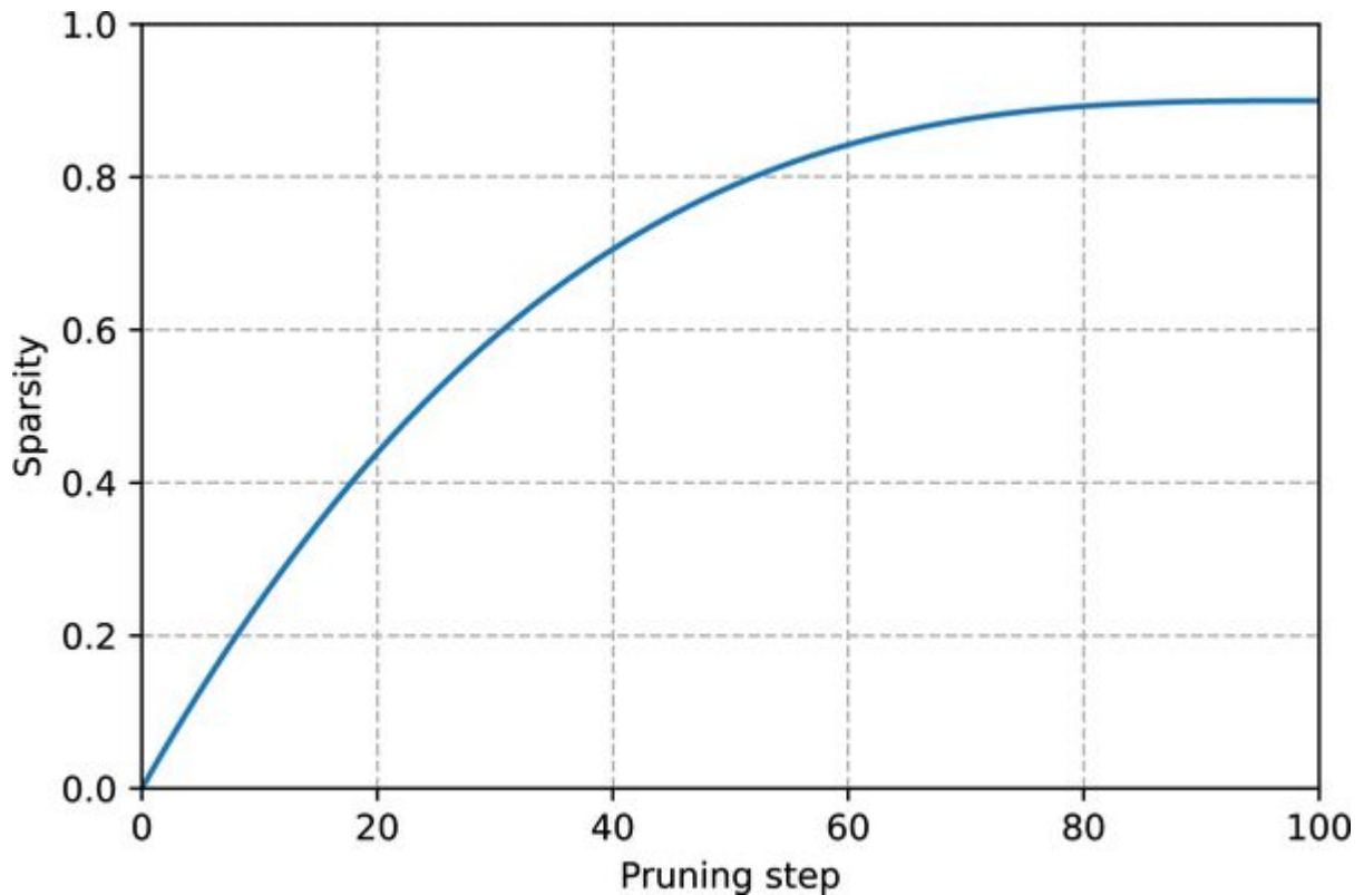
Figure 8-11. The cubic sparsity scheduler used for pruning
