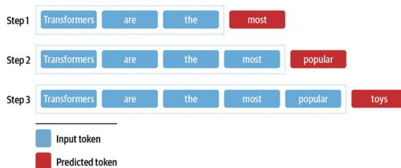
Figure 5-3. Generating text from an input sequence by adding a new word to the input at each step
