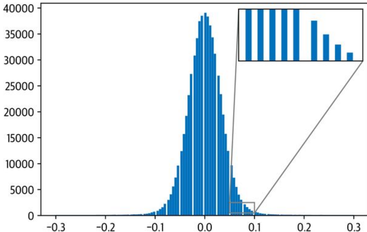
Figure 8-7. Effect of quantization on a transformer's weights
