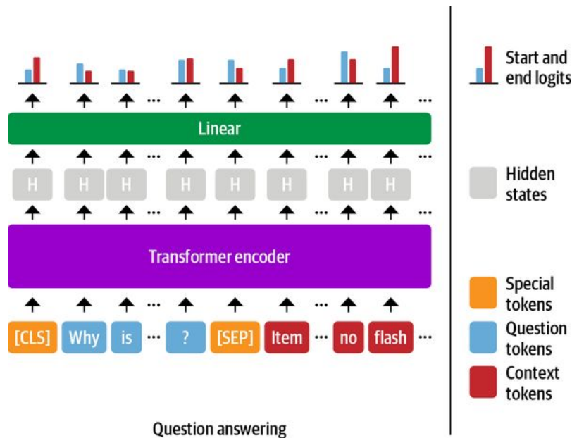
Figure 7-4. The span classification head for QA tasks
