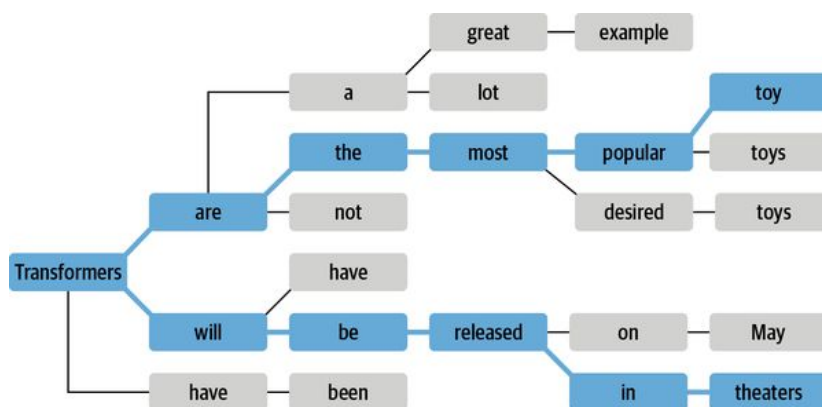
Figure 5-4. Beam search with two beams
