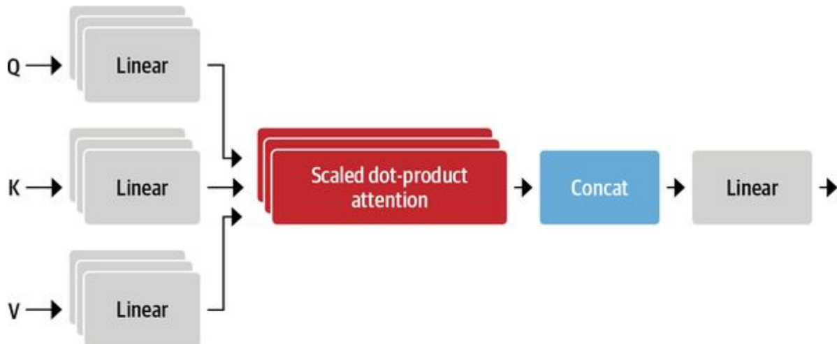
Figure 3-5. Multi-head attention
