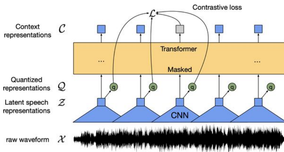
Figure 11-12. Architecture of wav2vec 2.0 (courtesy of Alexei Baevski)
