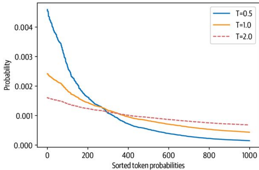
Figure 5-5. Distribution of randomly generated token probabilities for three selected temperatures
