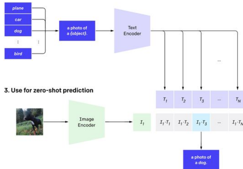
Figure 11-17. Architecture of CLIP (courtesy of Alec Radford)
