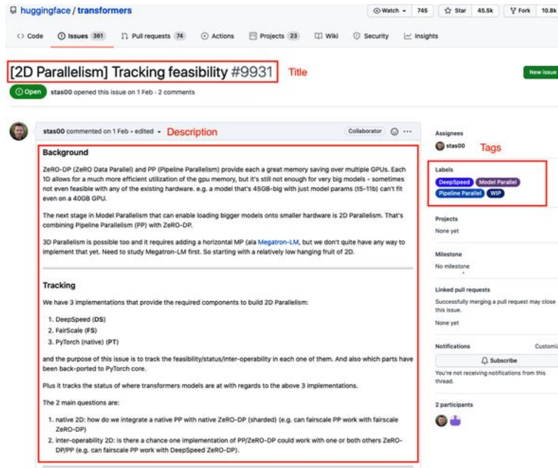
Figure 9-2. A typical GitHub issue on the 🤖 Transformers repository
