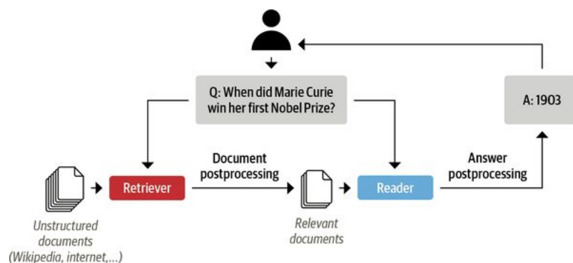
Figure 7-9. The retriever-reader architecture for modern QA systems
