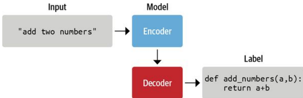
Figure 10-4. Using an encoder-decoder architecture for a sequence-to-sequence task where the inputs are split into comment/code pairs using heuristics: the model gets one element as input and needs to generate the other one
