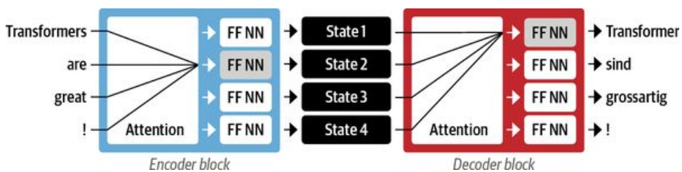
Figure 1-6. Encoder-decoder architecture of the original Transformer
