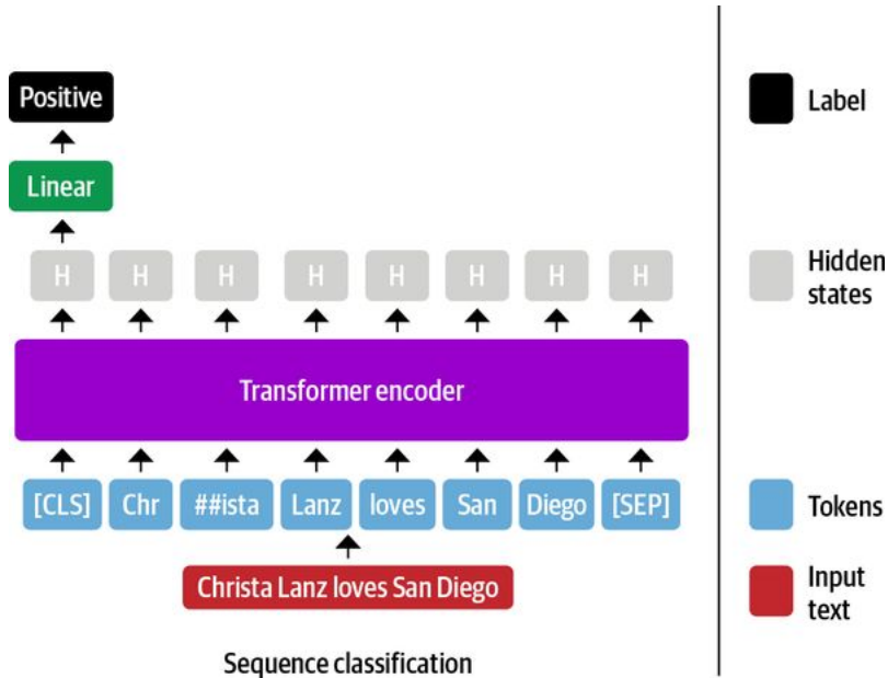
Figure 4-2. Fine-tuning an encoder-based transformer for sequence classification
