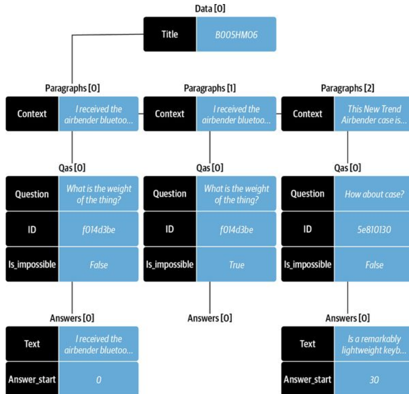
Figure 7-11. Visualization of the SQuAD JSON format
